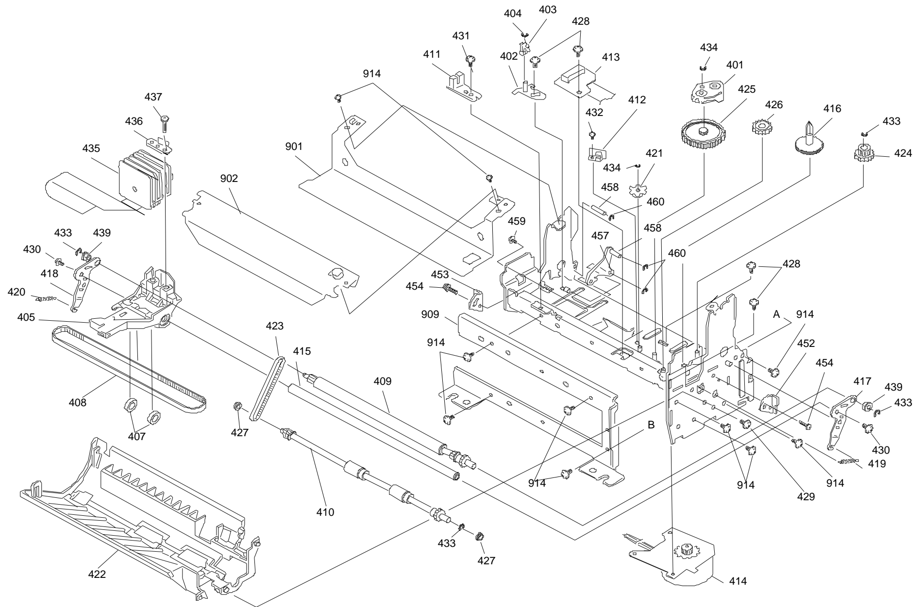
EXPLODED DIAGRAM FOR TM-U950 NO.2
