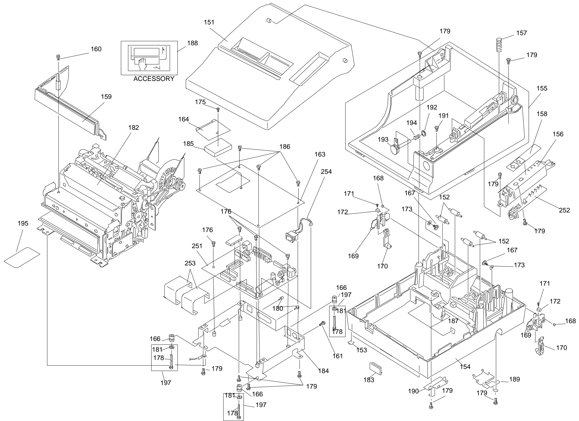
EXPLODED DIAGRAM FOR TM-U950 No.1
