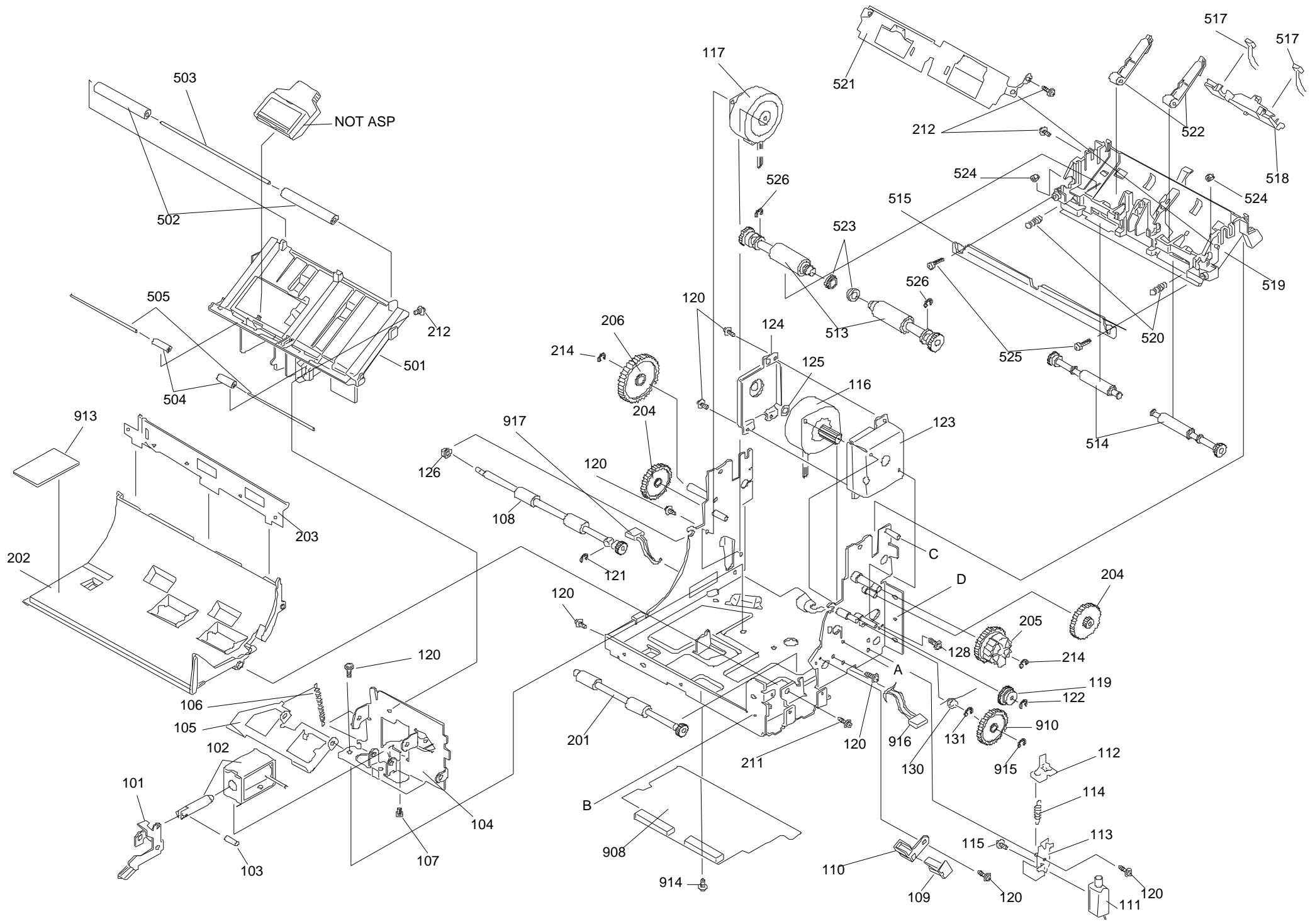
EXPLODE DIAGRAM FOR TM-U950 NO.4
